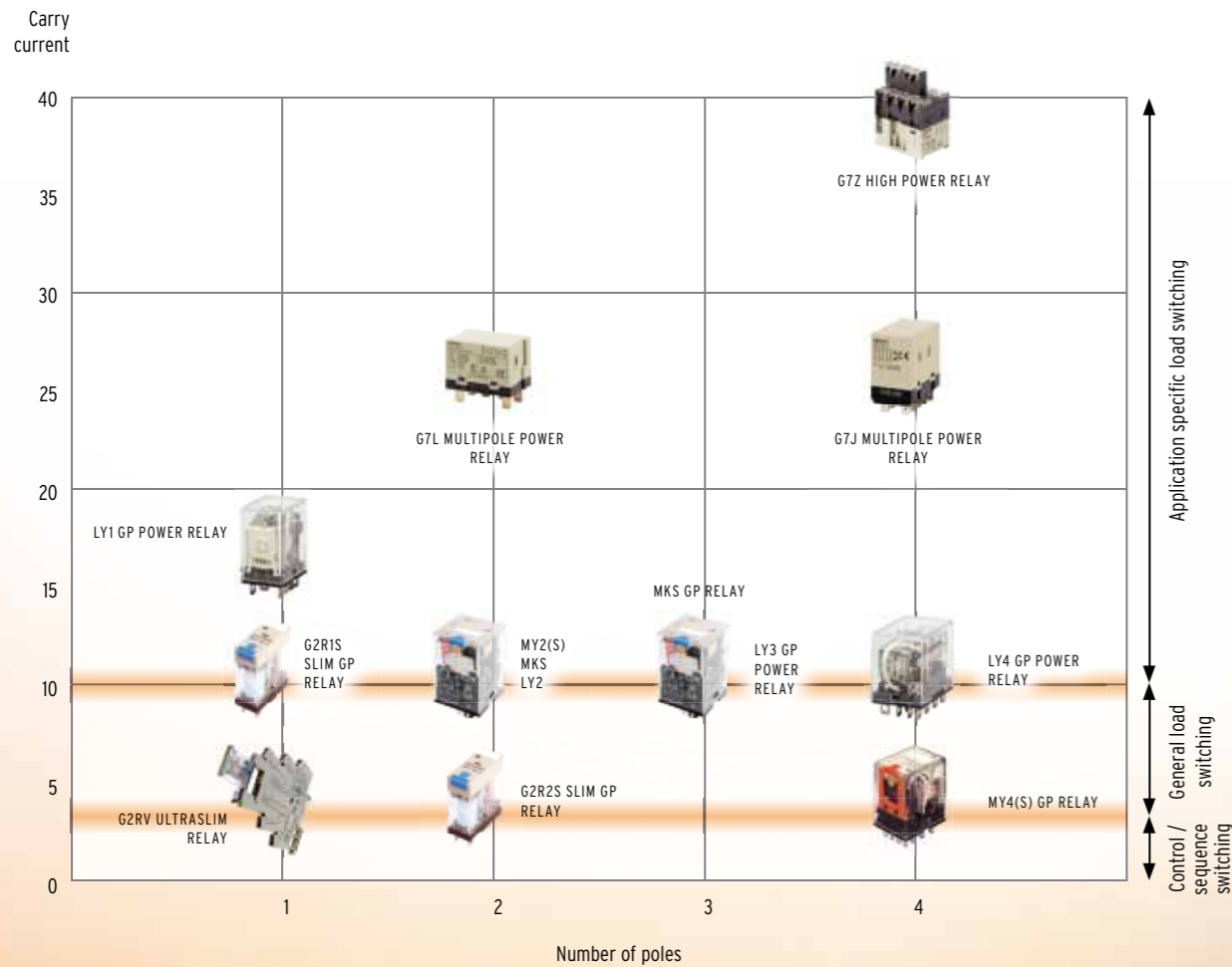
Electromechanical relay portfolio
