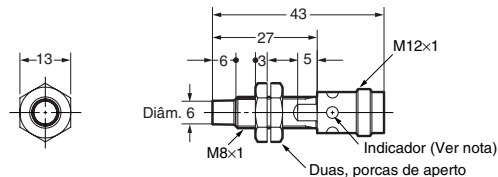
E2A-S08KN04-M1-□□
