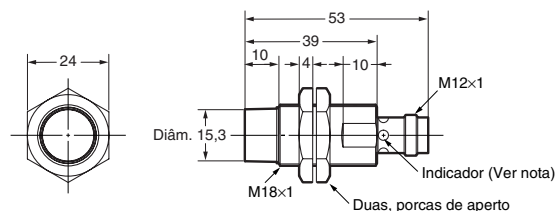
E2A-M18KN16-M1-□□/E2A-S18KN16-M1-□
