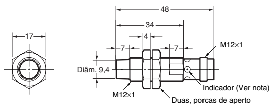
E2A-M12KN08-M1-□□/E2A-S12KN08-M1-□
