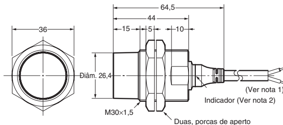
E2A-M30KN20-WP-□□/E2A-S30KN20-WP-□
