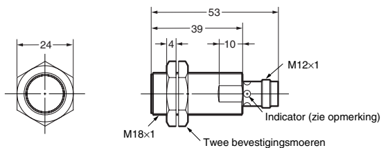
E2A-M18KS08-M1-□□/E2A-S18KS08-M1-□
