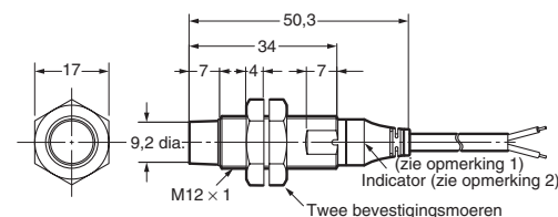
E2A-M12KN08-WP-□□/E2A-S12KN08-WP-□
