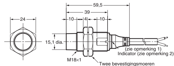
E2A-M18KN16-WP-□□/E2A-S18KN16-WP-□
