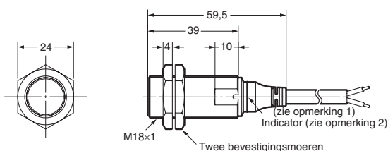
E2A-M18KS08-WP-□□/E2A-S18KS08-WP-□
