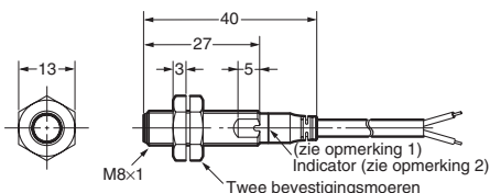
E2A-S08KS02-WP-□□
