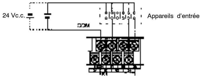
CPM1A-20CDR-□/20CDT-D/20CDT1-D CPM1A-20EDR/20EDT/20EDT1
