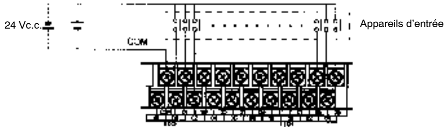
CPM1A-30CDR-□/30CDT-D/30CDT1-D
