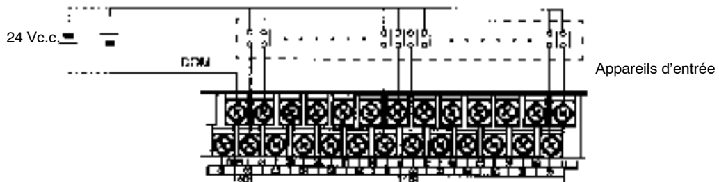
CPM1A-40CDR-□/40CDT-D/40CDT1-D
