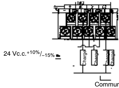
CPM1A-20CDT-D/CPM1A-20EDT
