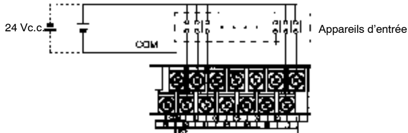
CPM1A-20CDR-□/20CDT-D/20CDT1-D CPM1A-20EDR/20EDT/20EDT1
