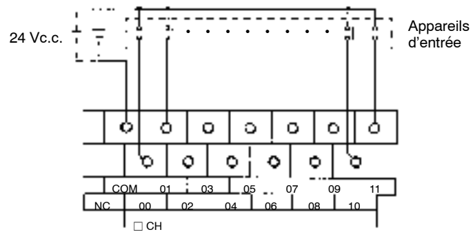
CPM1A-20EDR/20EDR1/EDT/EDT1
