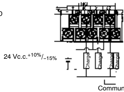
CPM1A-20CDT1-D/CPM1A-20EDT1
